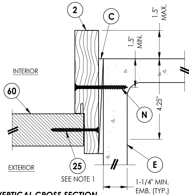
1 8 VERTICAL CROSS SECTION Shown Direct to Masonry Outswing only w/ 6-9/16" jamb
